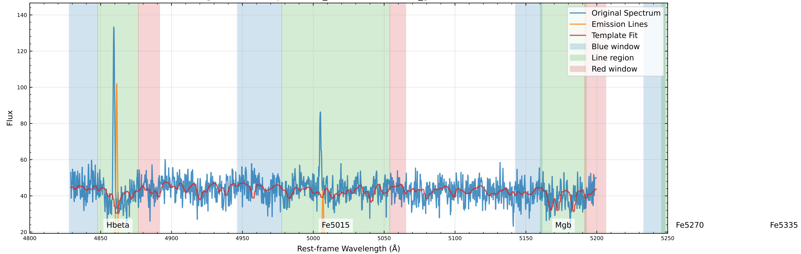
Original Data Comparison (v_star=-109.0 km/s, v_gas=-120.6 km/s)
