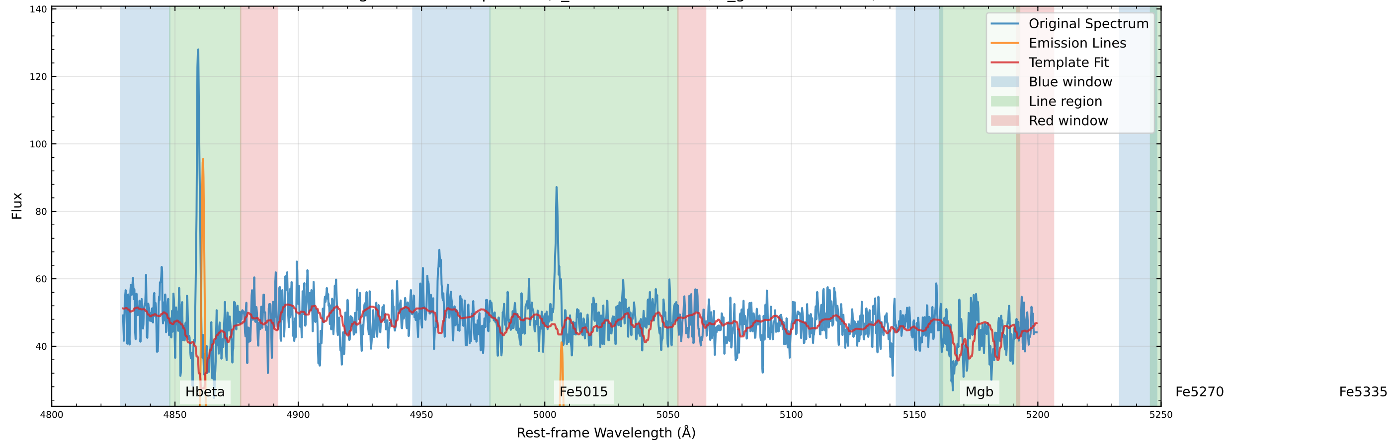
Original Data Comparison (v_star=-117.7 km/s, v_gas=-118.9 km/s)
