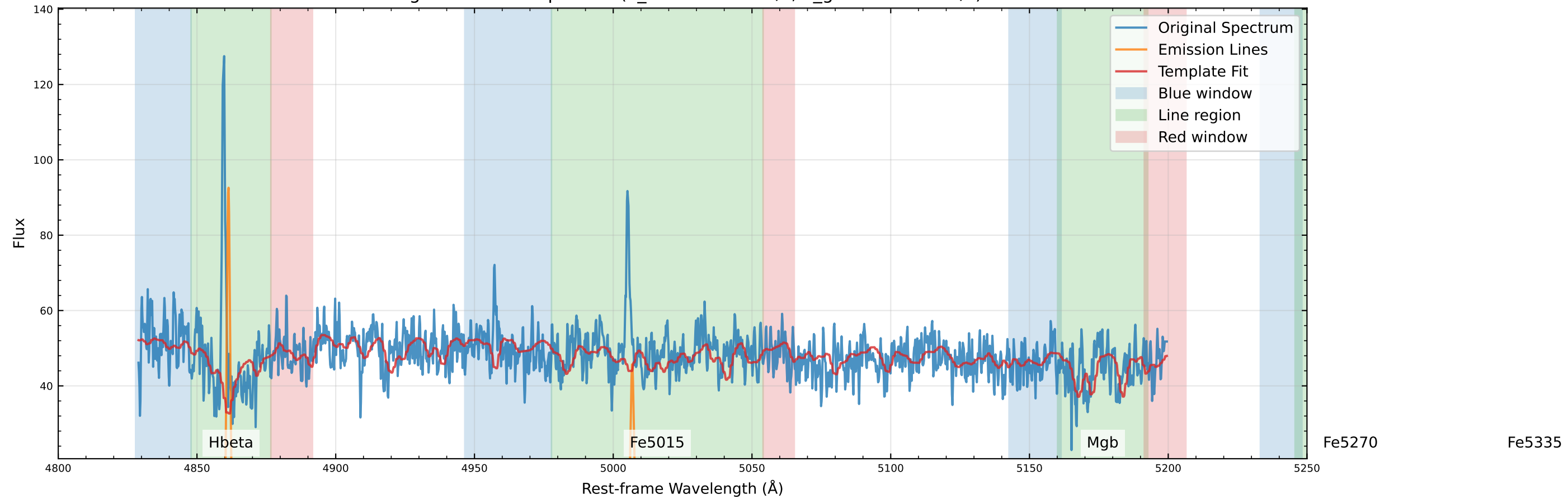
Original Data Comparison ( v_{\text{star}}=-91.8 km/s, v_{\text{gas}}=-104.1 km/s)
