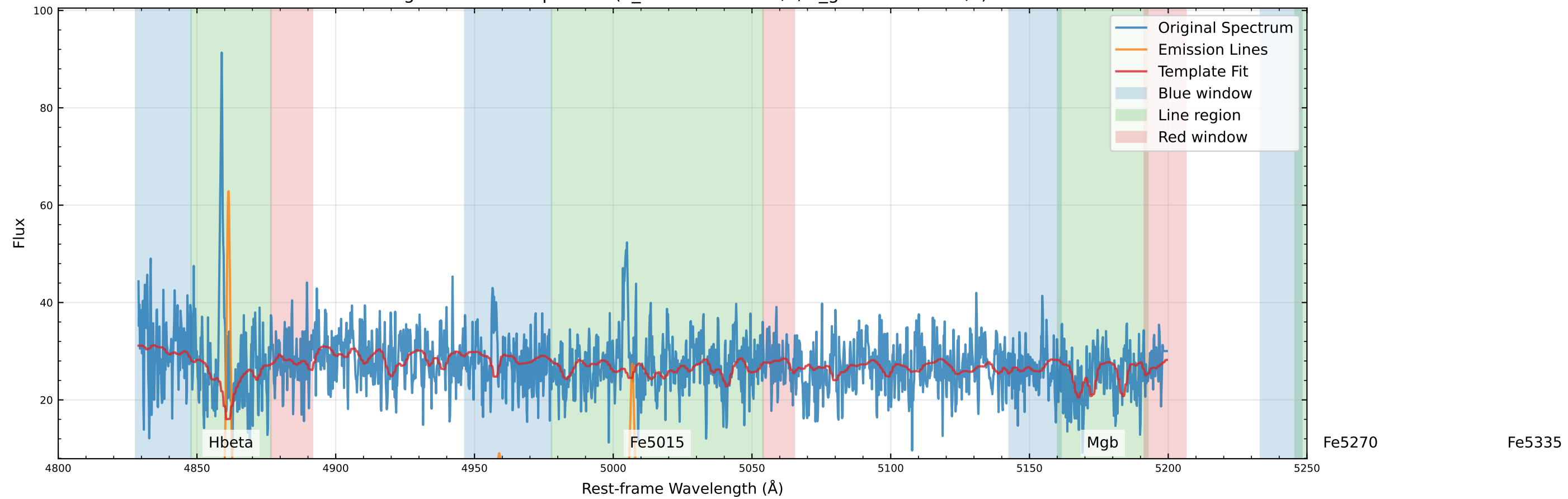
Original Data Comparison (v_star=-151.1 km/s, v_gas=-150.7 km/s)
