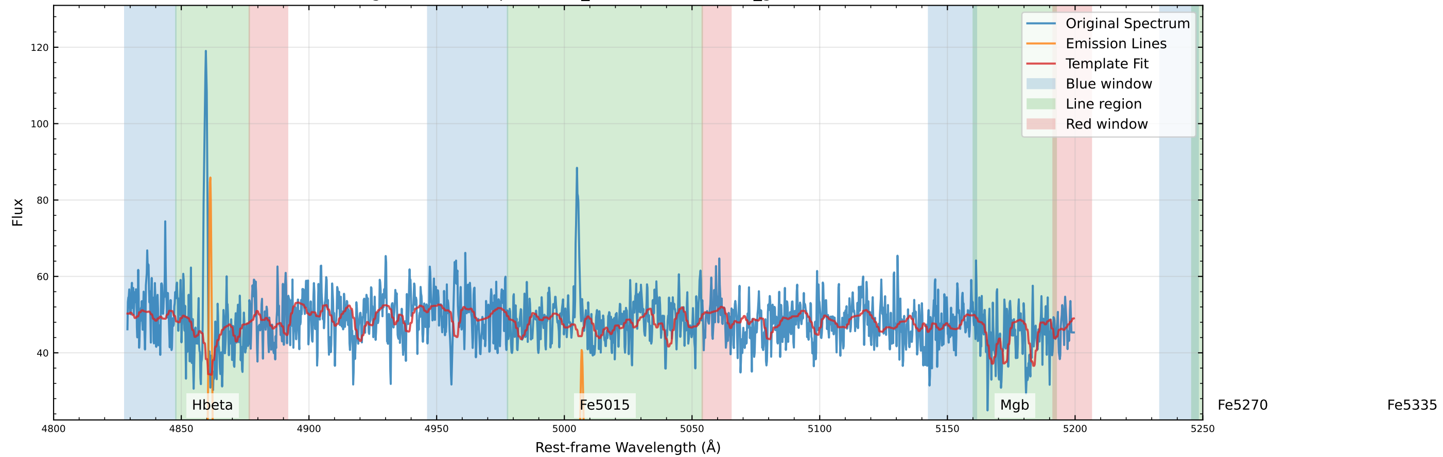
Original Data Comparison (v_star=-113.0 km/s, v_gas=-108.8 km/s)
