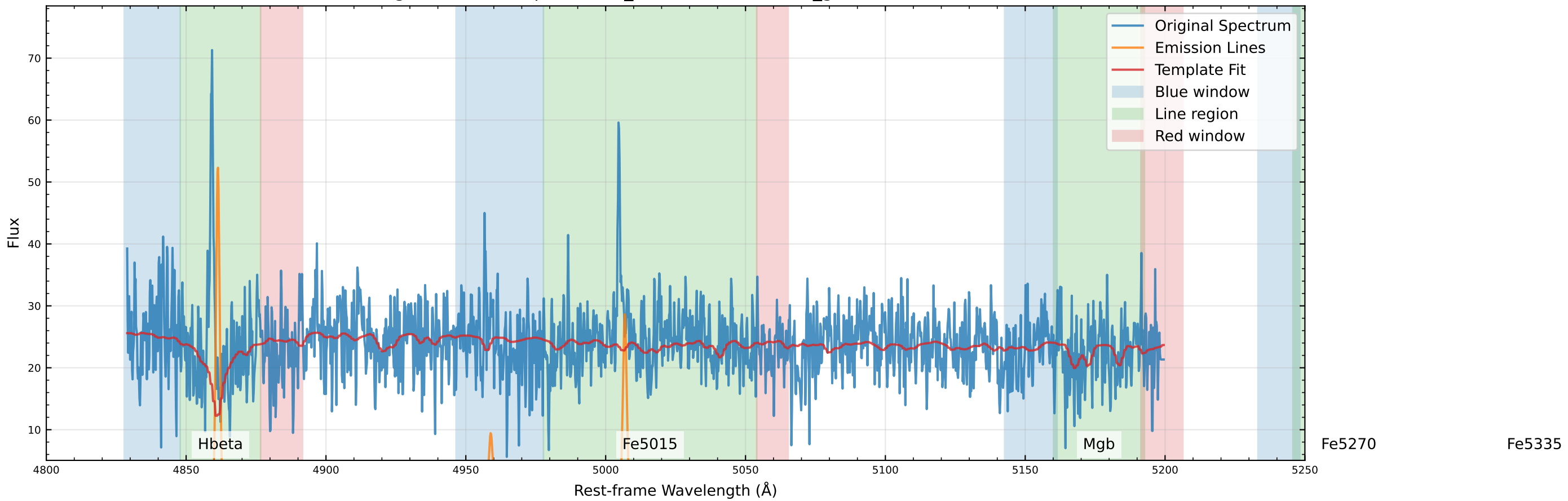
Original Data Comparison (v_star=-127.6 km/s, v_gas=-129.3 km/s)
