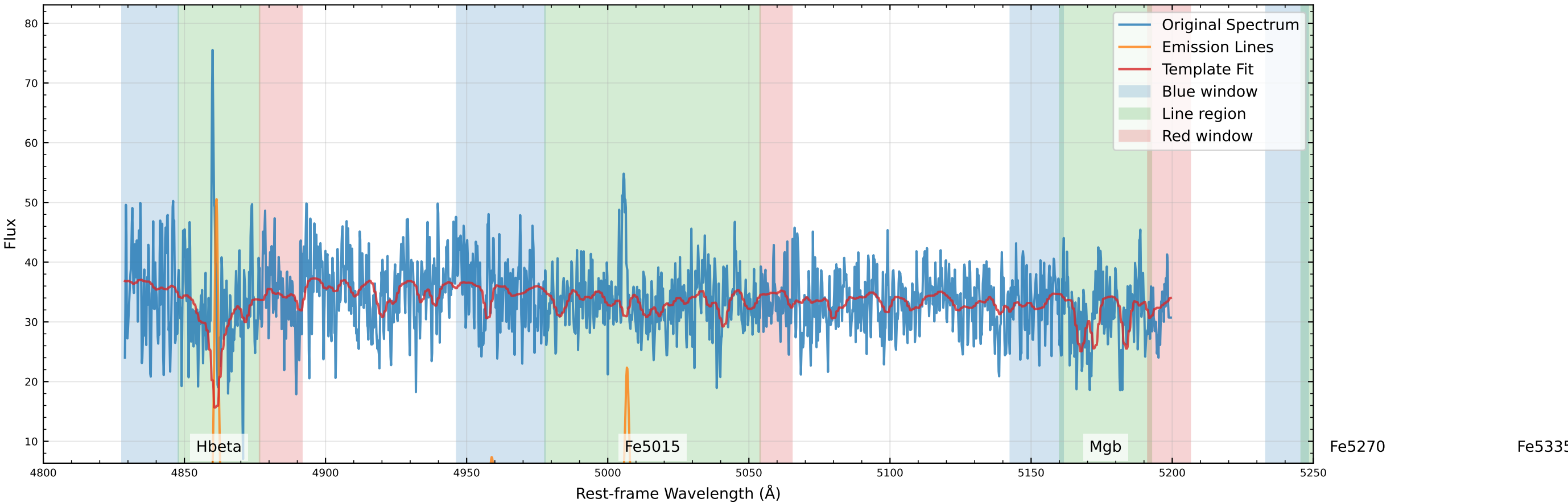
Original Data Comparison (v_star=-89.3 km/s, v_gas=-74.9 km/s)
