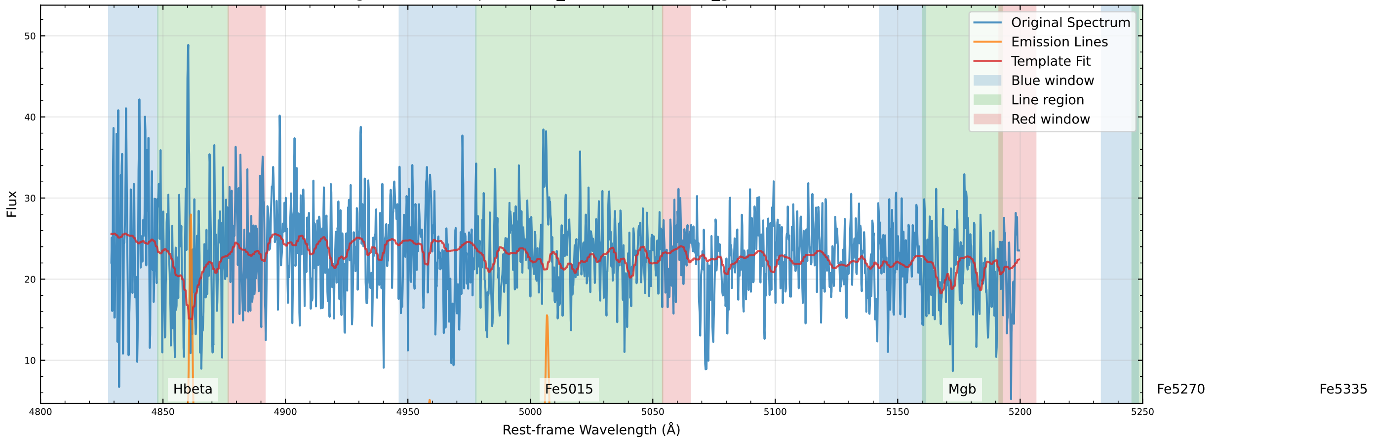
Original Data Comparison (v_star=-58.5 km/s, v_gas=-71.4 km/s)
