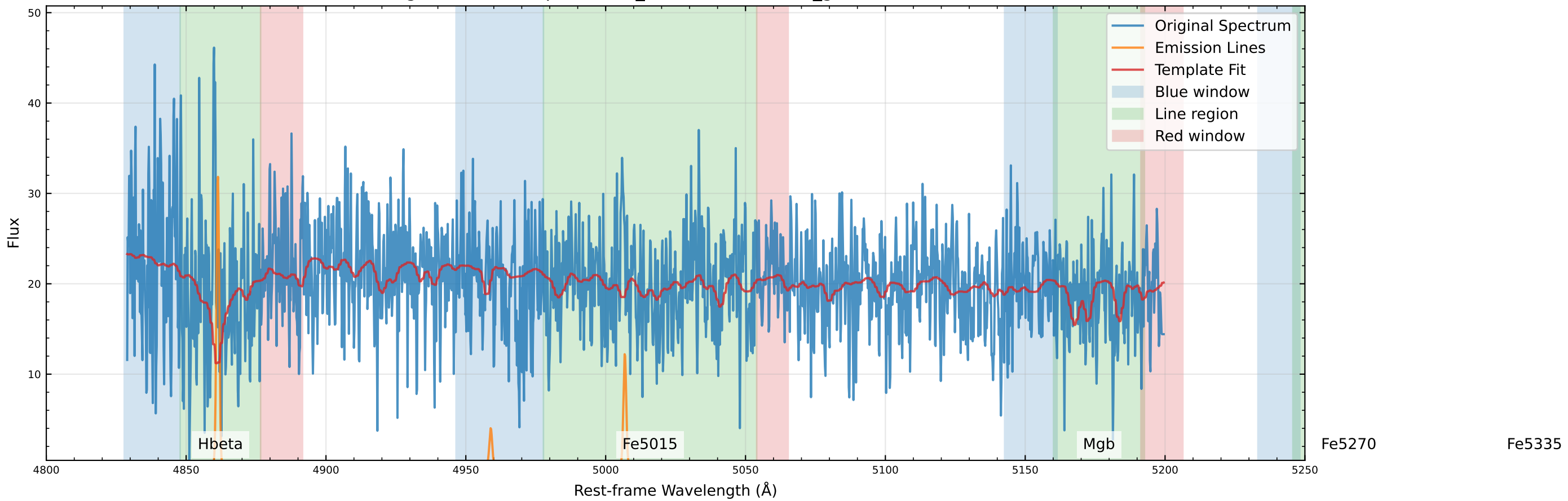
Original Data Comparison (v_star=-88.6 km/s, v_gas=-75.5 km/s)
