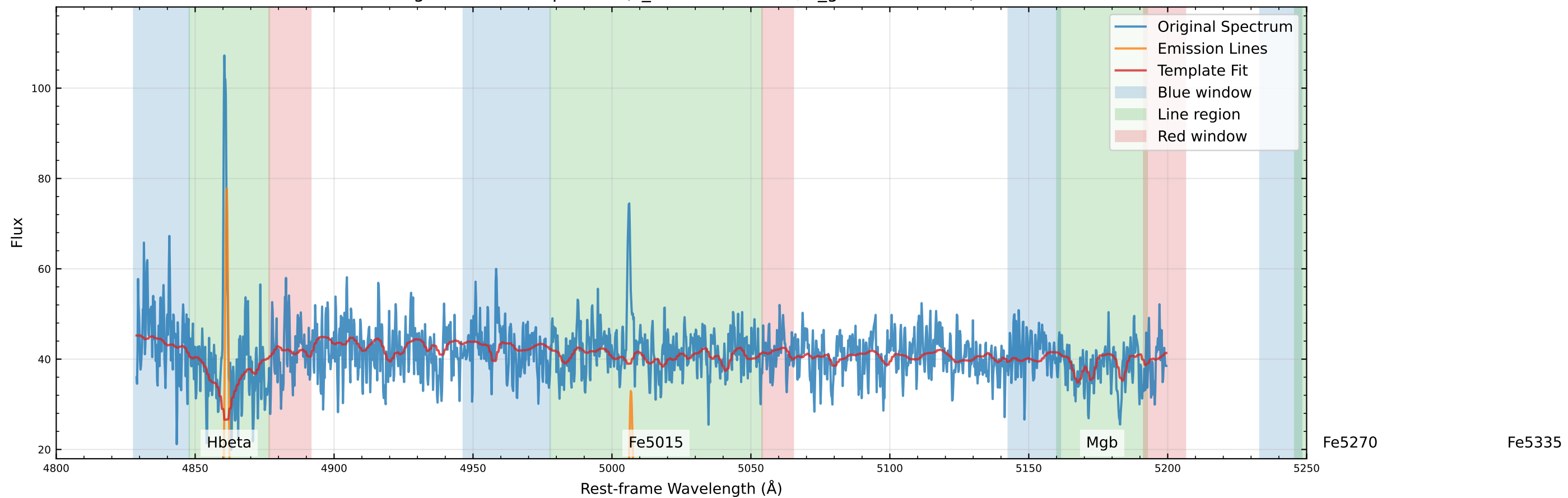
Original Data Comparison (v_star=-59.7 km/s, v_gas=-37.8 km/s)
