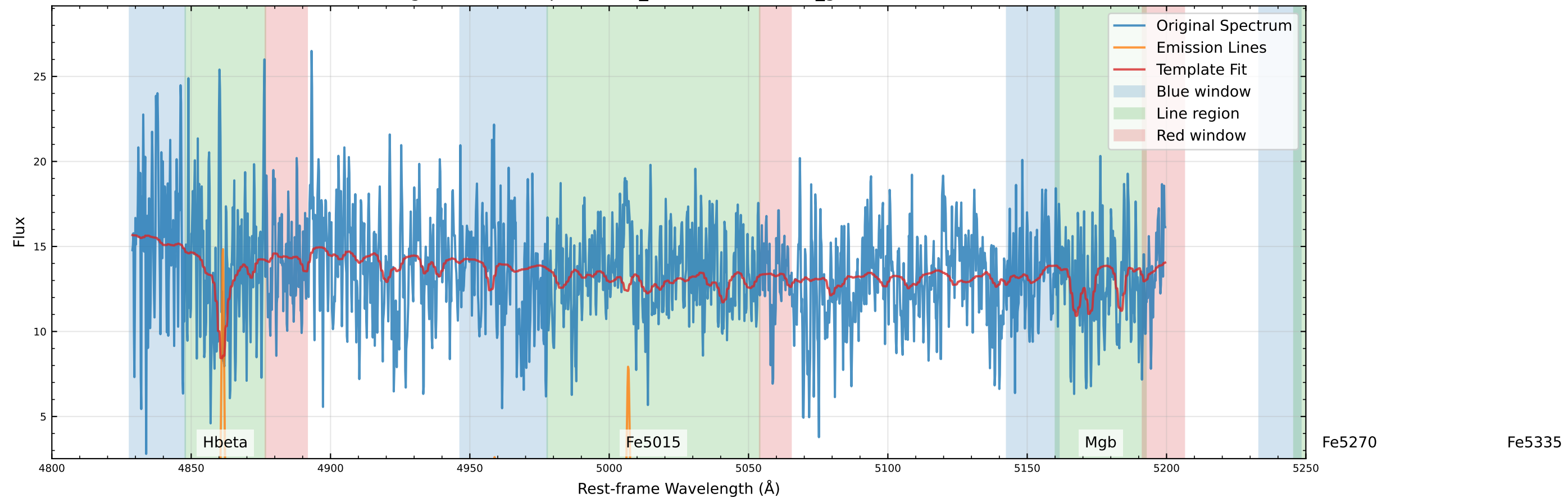
Original Data Comparison (v_star=-61.2 km/s, v_gas=-64.4 km/s)
