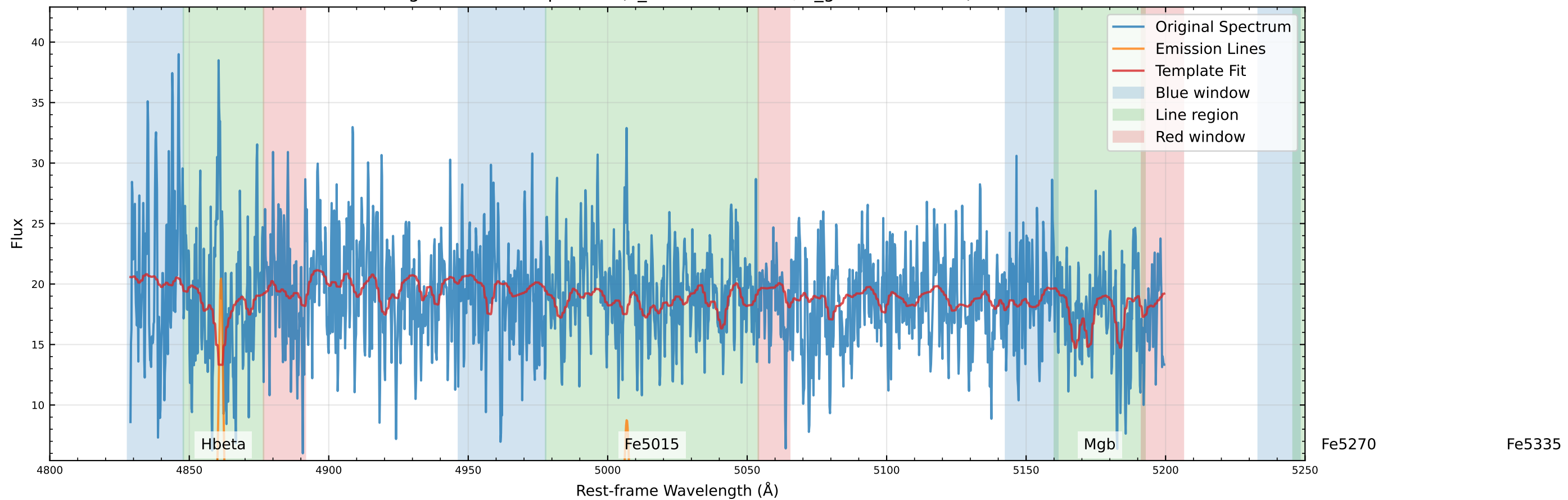
Original Data Comparison (v_star=-32.5 km/s, v_gas=-40.4 km/s)
