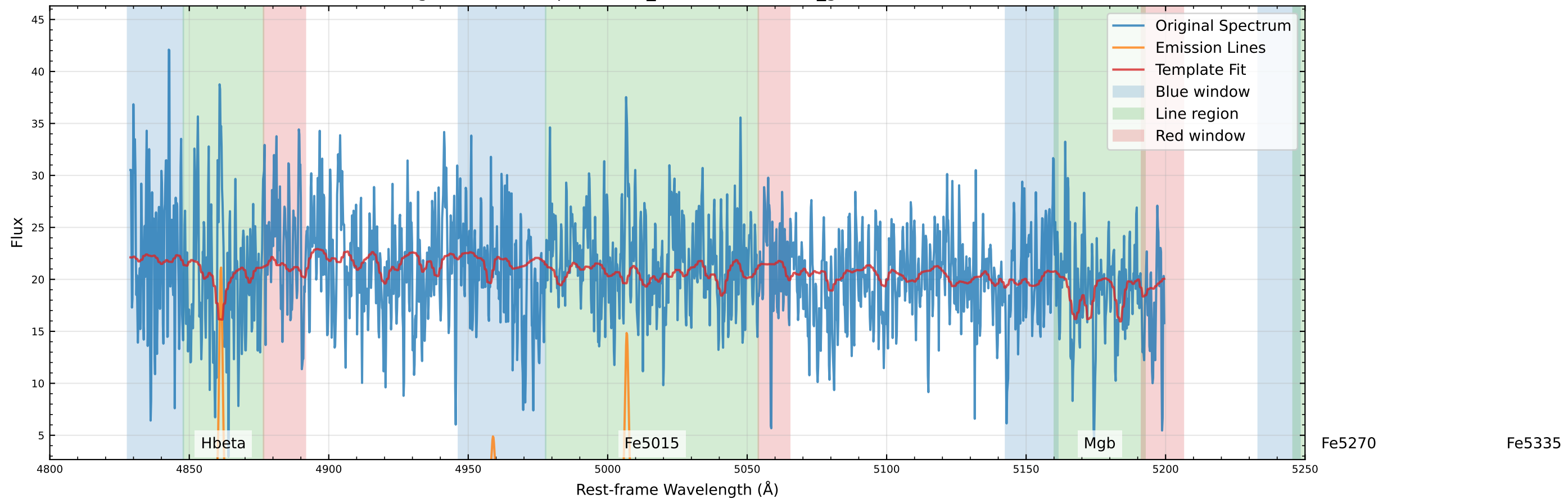
Original Data Comparison (v_star=26.3 km/s, v_gas=-6.5 km/s)
