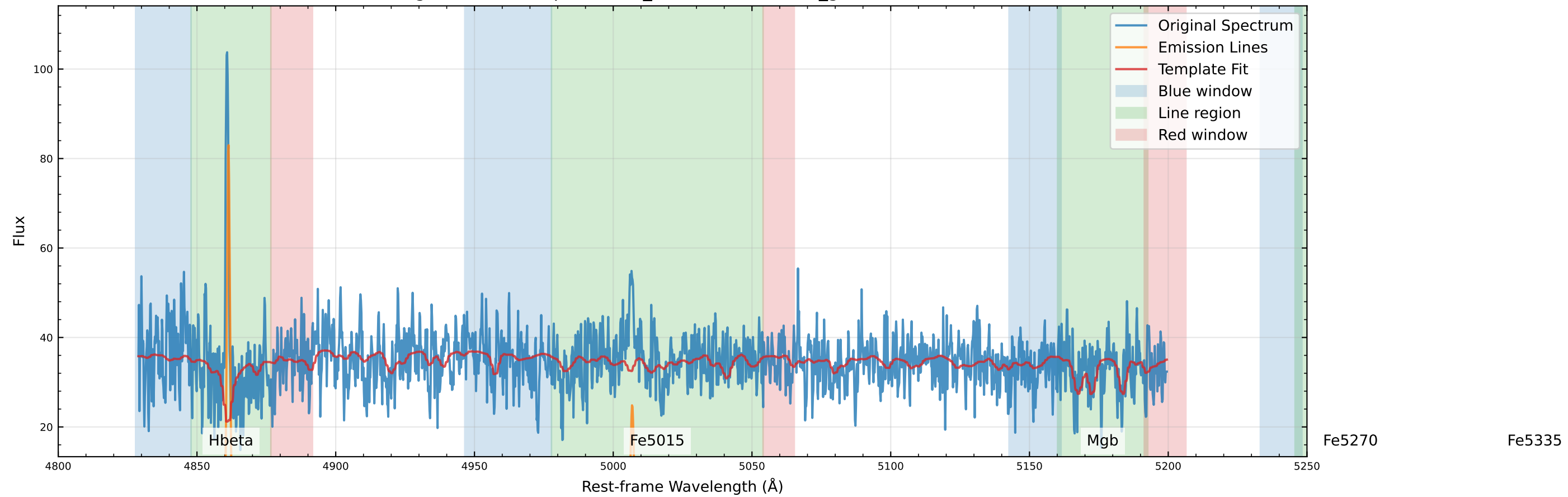
Original Data Comparison (v_star=-29.5 km/s, v_gas=-30.6 km/s)
