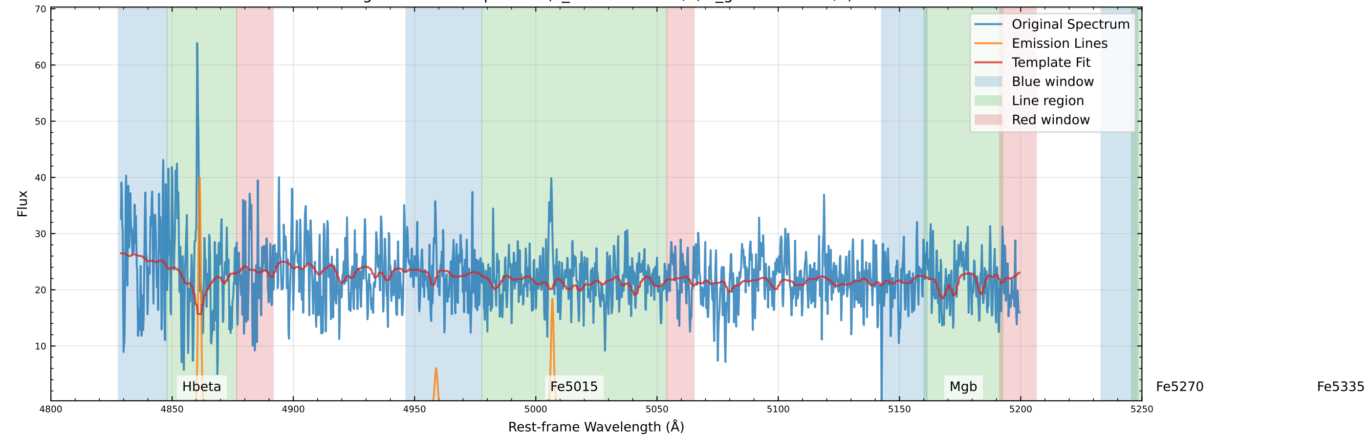
Original Data Comparison (v_star=-57.9 km/s, v_gas=-50.3 km/s)
