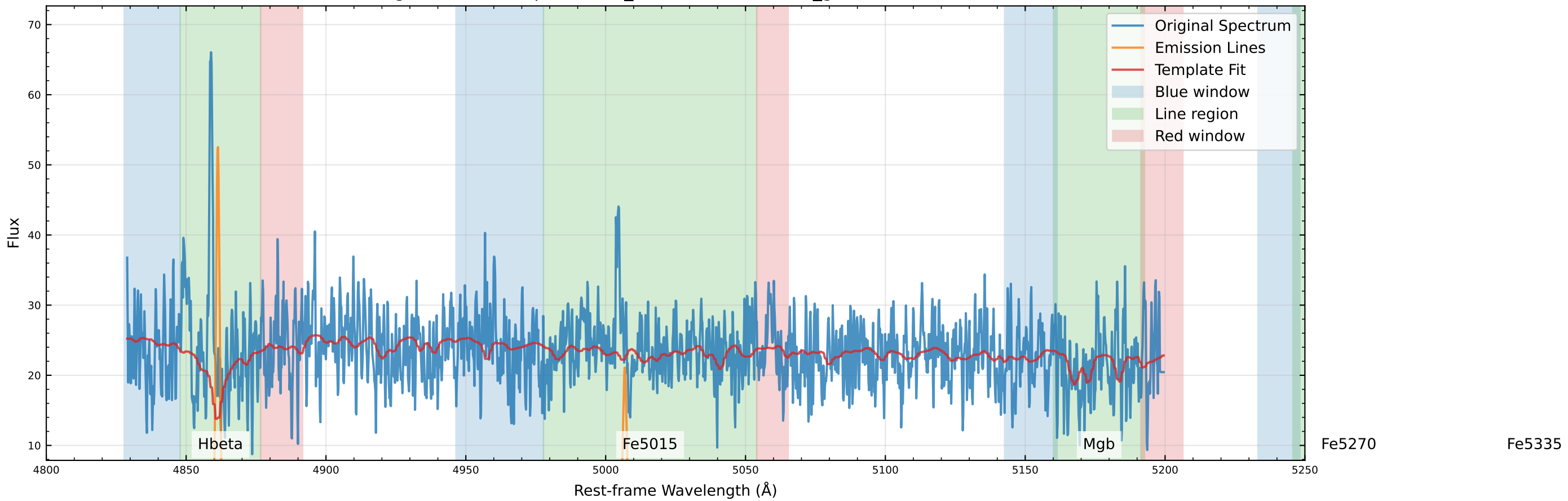
Original Data Comparison (v_star=-137.8 km/s, v_gas=-150.9 km/s)
