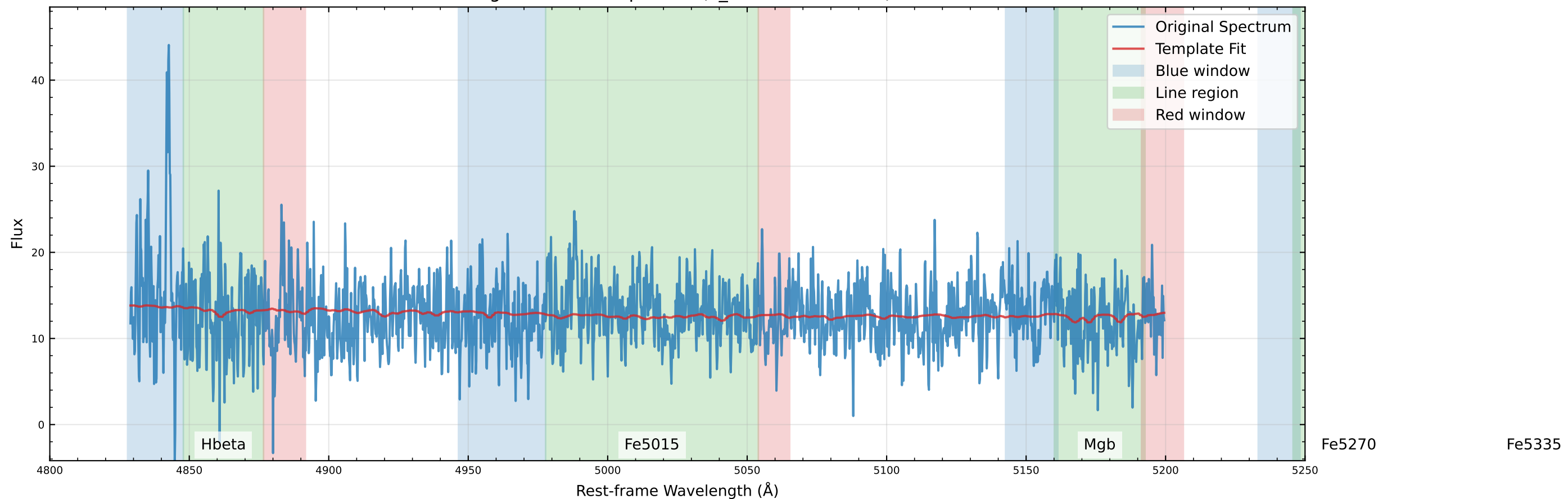
Original Data Comparison (v_star=-162.9 km/s)
