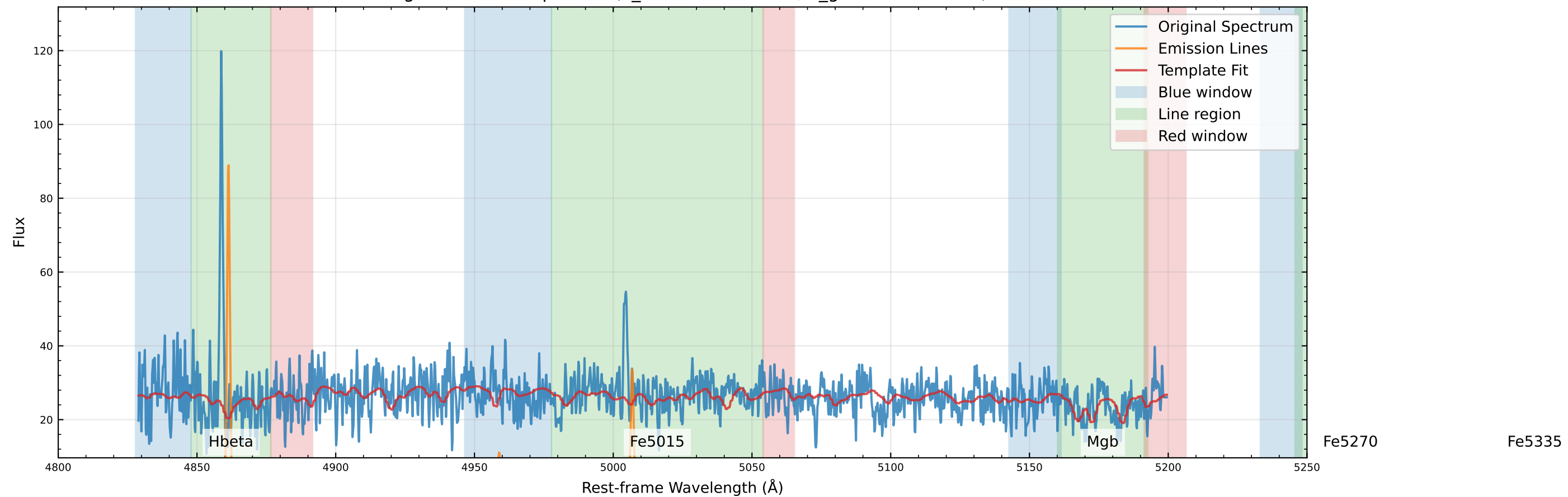
Original Data Comparison (v_star=-140.7 km/s, v_gas=-155.2 km/s)
