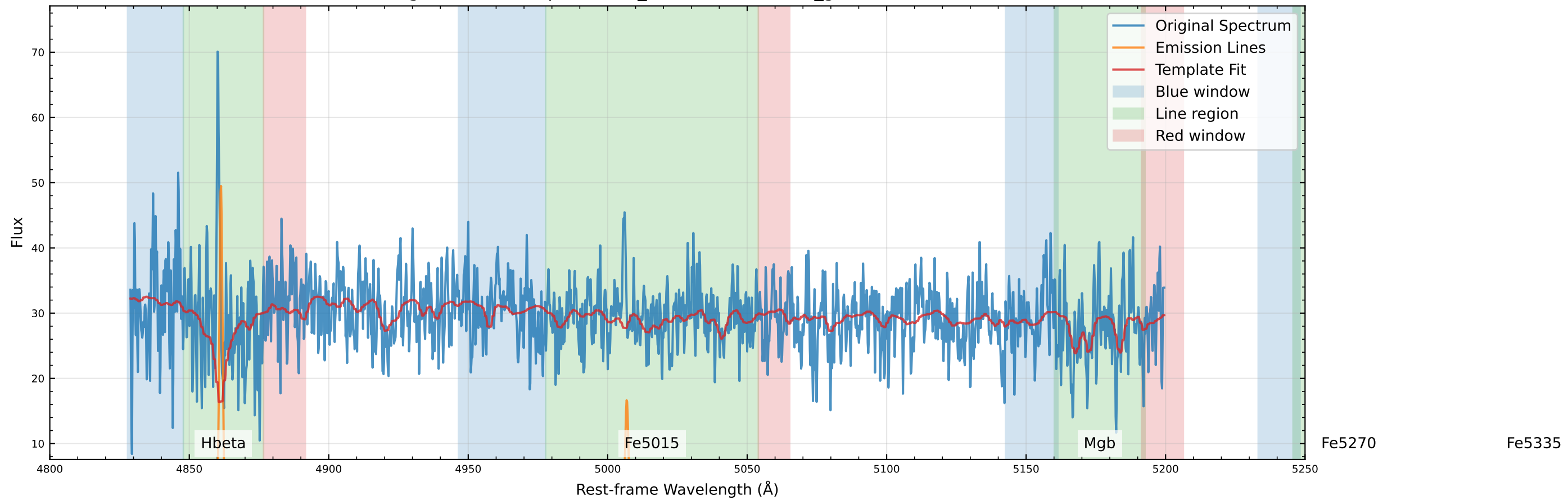
Original Data Comparison (v_star=-56.4 km/s, v_gas=-60.6 km/s)
