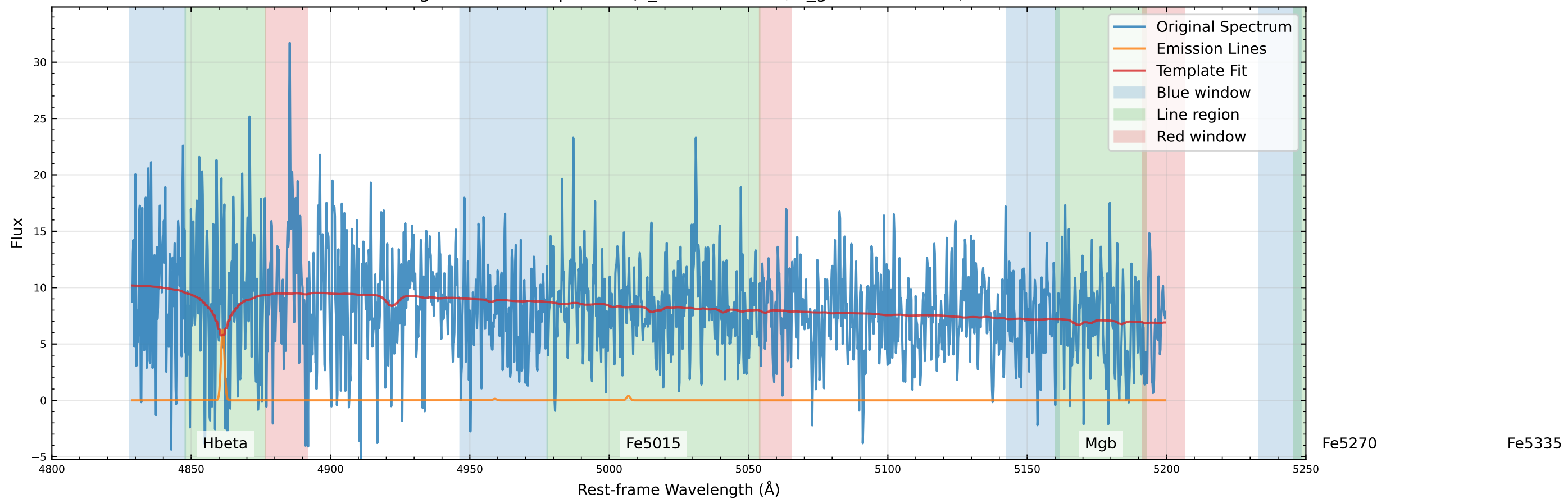
Original Data Comparison (v_star=0.0 km/s, v_gas=-29.6 km/s)
