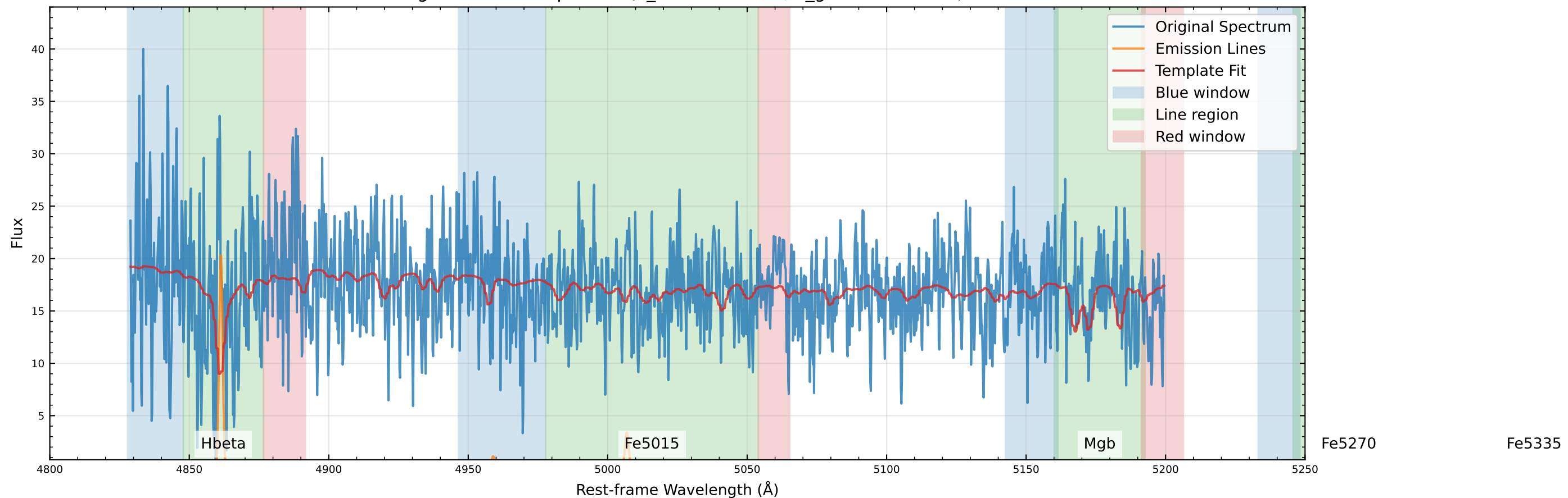
Original Data Comparison (v_star=4.1 km/s, v_gas=-31.1 km/s)
