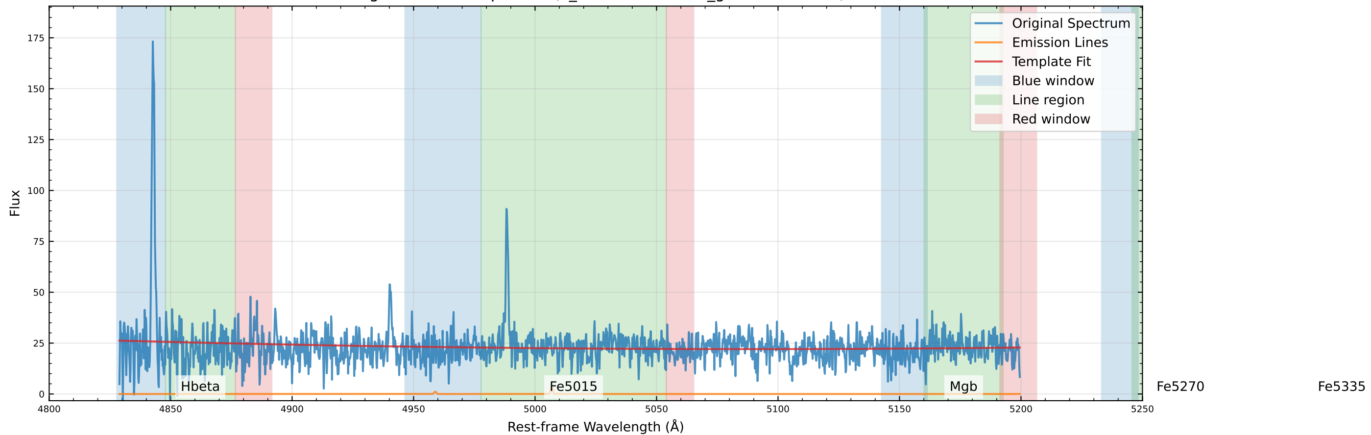
Original Data Comparison (v_star=0.0 km/s, v_gas=-41.9 km/s)
