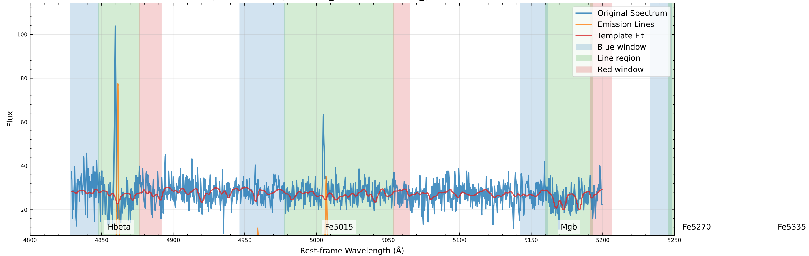
Original Data Comparison (v_star=-70.1 km/s, v_gas=-113.5 km/s)
