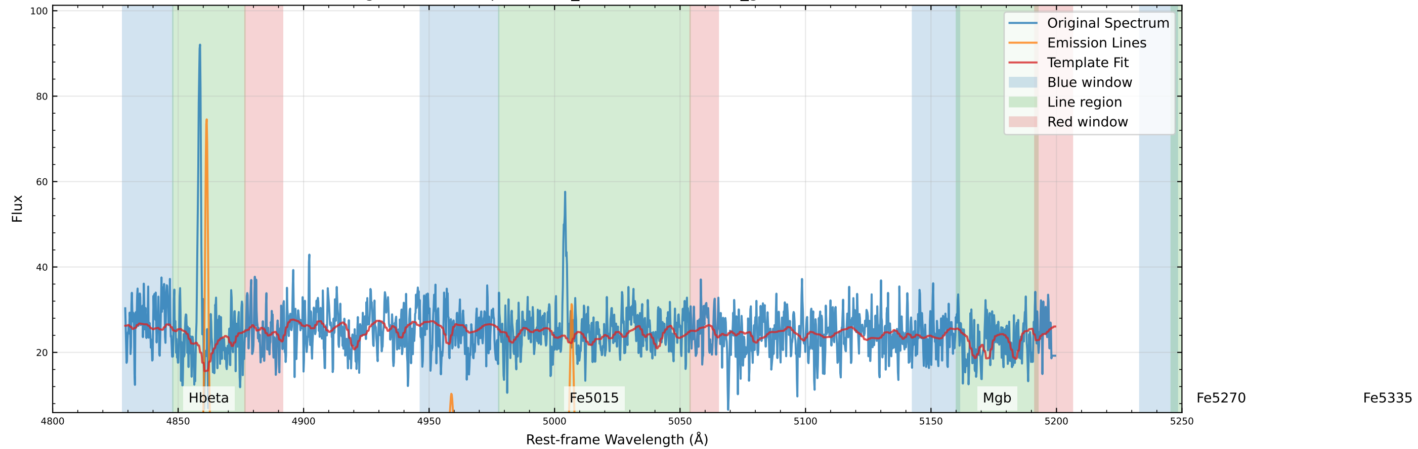
Original Data Comparison (v_star=-152.9 km/s, v_gas=-170.0 km/s)
