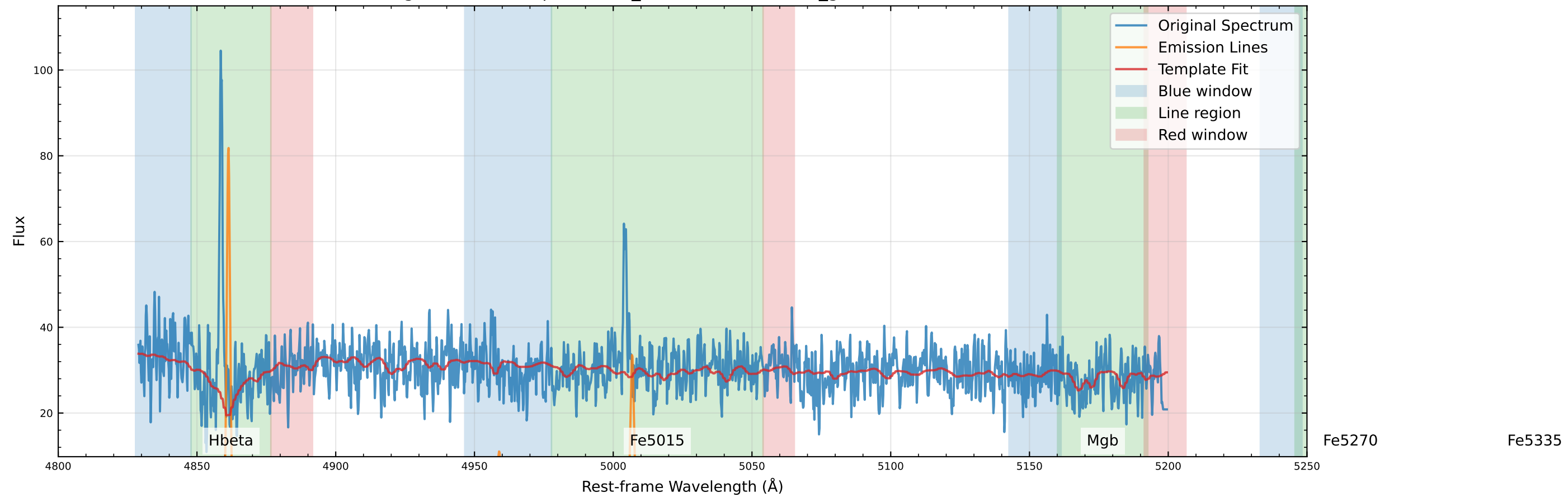
Original Data Comparison (v_star=-171.0 km/s, v_gas=-163.3 km/s)
