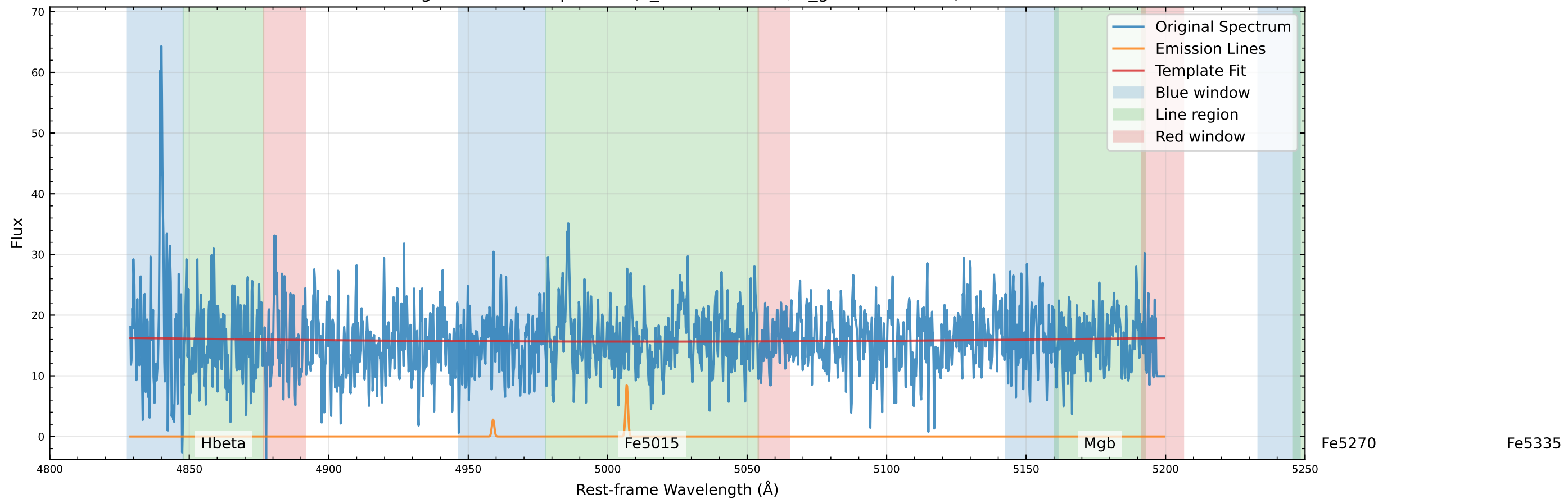
Original Data Comparison (v_star=0.0 km/s, v_gas=89.8 km/s)
