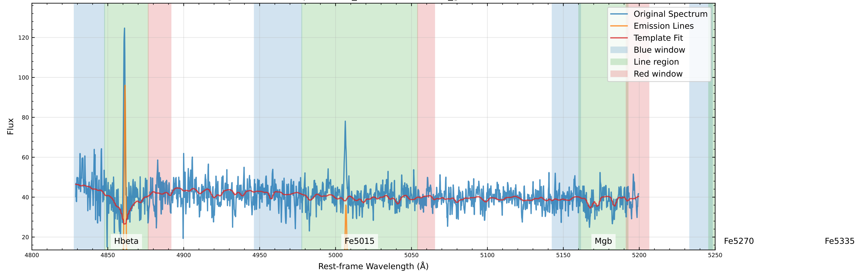
Original Data Comparison (v_star=-39.9 km/s, v_gas=-27.3 km/s)
