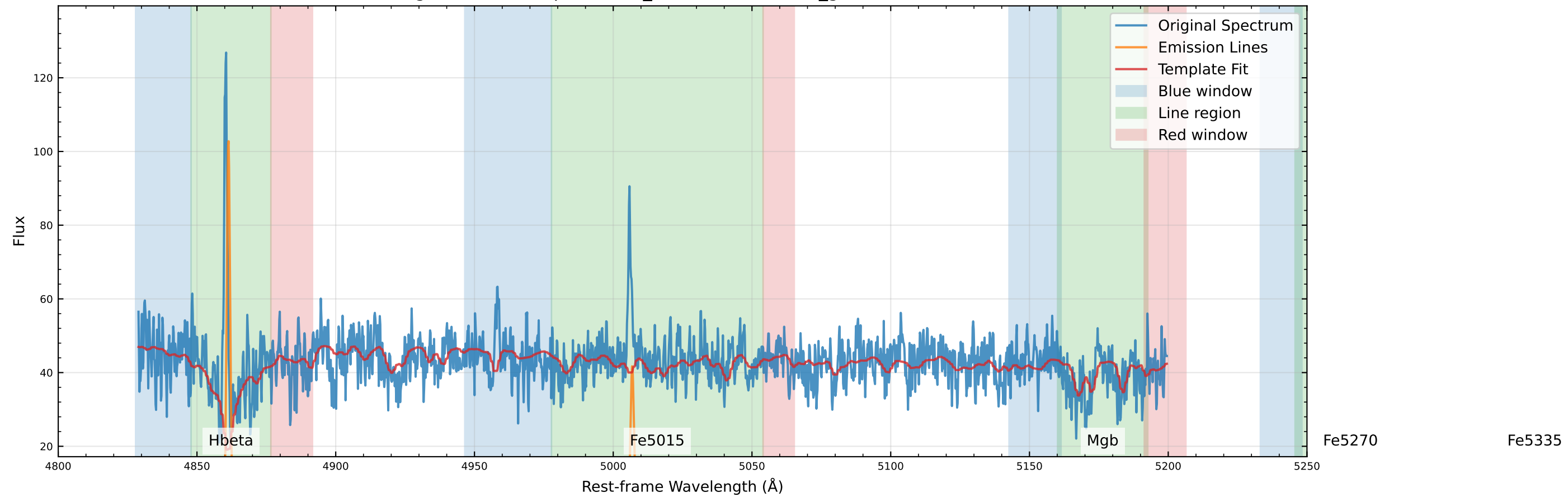
Original Data Comparison (v_star=-61.6 km/s, v_gas=-60.1 km/s)
