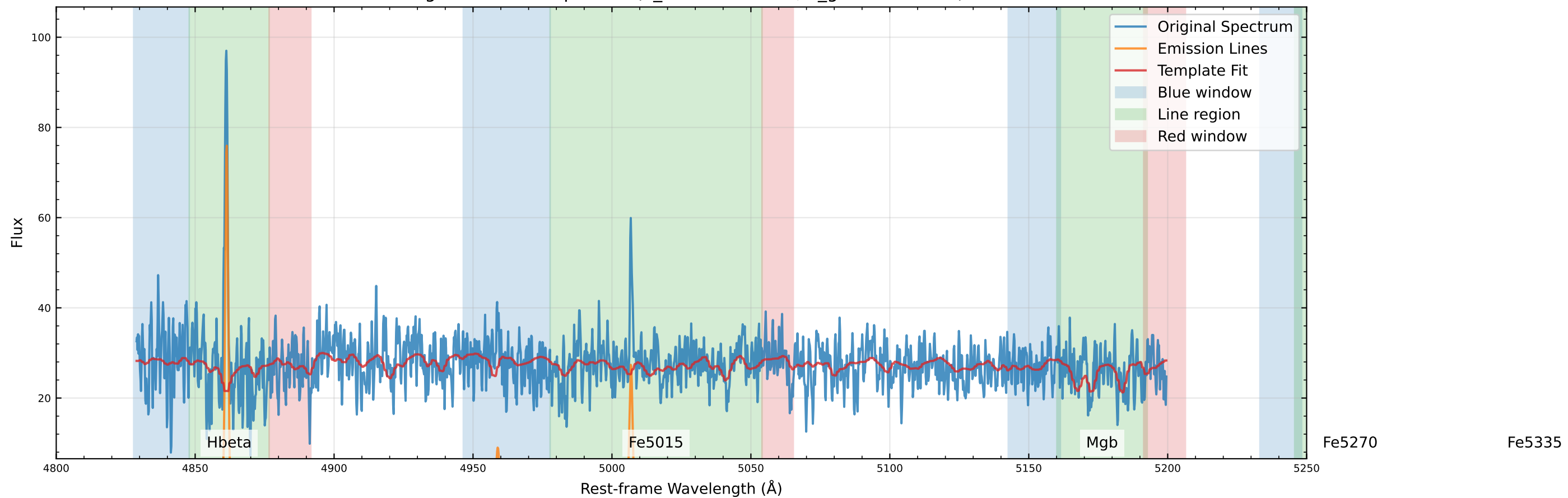
Original Data Comparison (v_star=-5.4 km/s, v_gas=-9.4 km/s)
