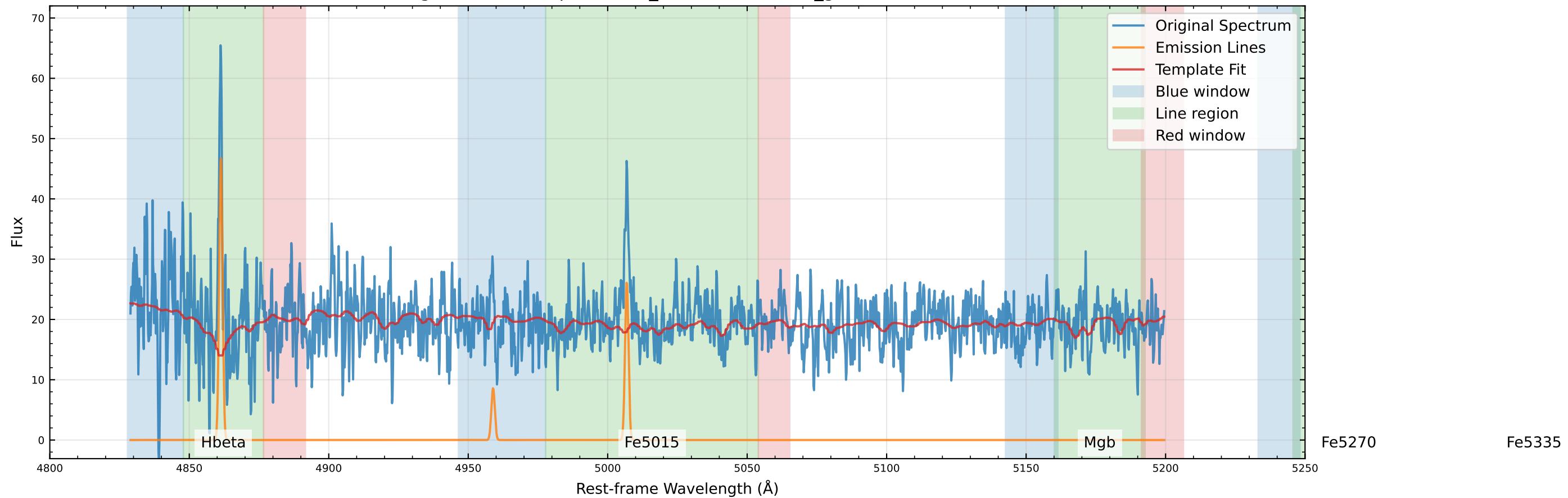
Original Data Comparison (v_star=-7.2 km/s, v_gas=-9.7 km/s)
