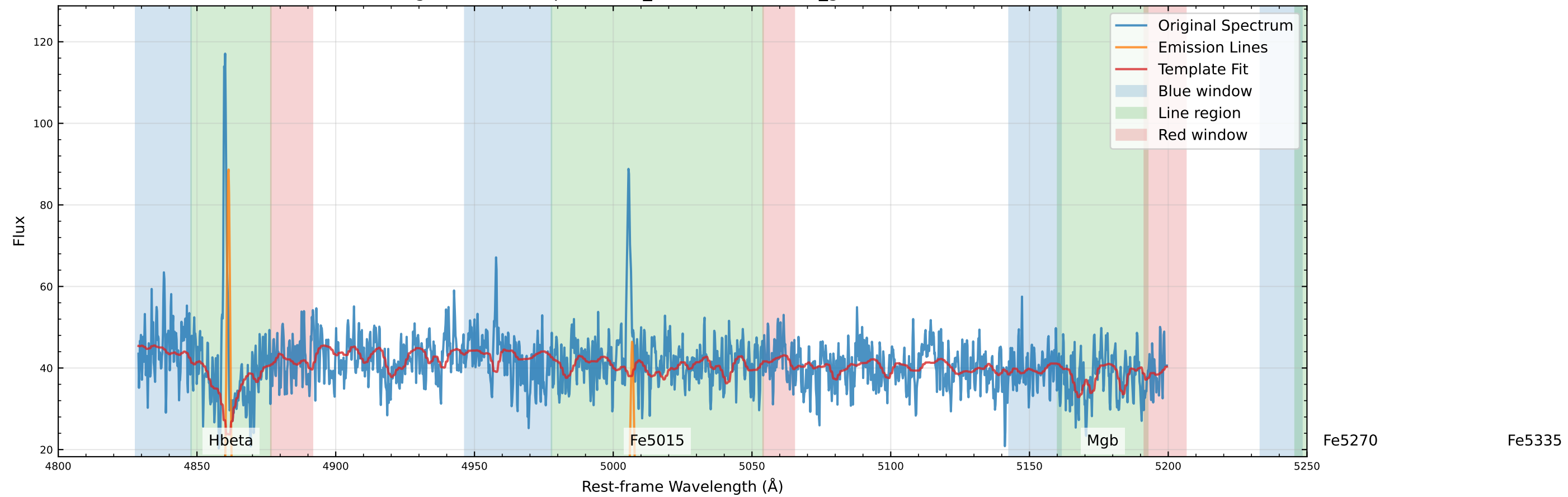
Original Data Comparison (v_star=-89.5 km/s, v_gas=-76.1 km/s)
