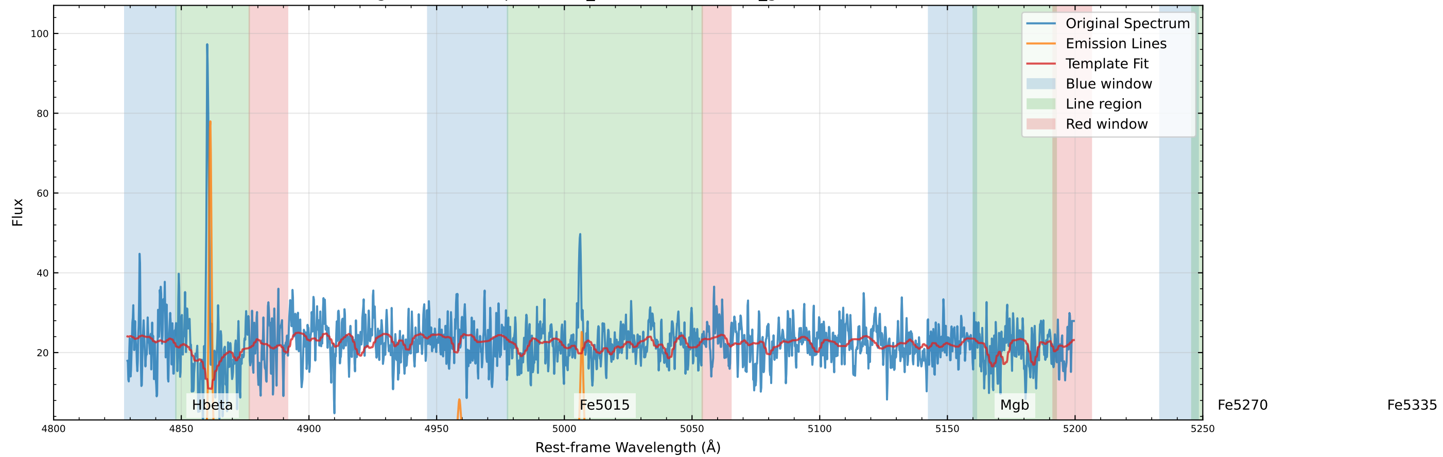
Original Data Comparison (v_star=-103.3 km/s, v_gas=-60.8 km/s)
