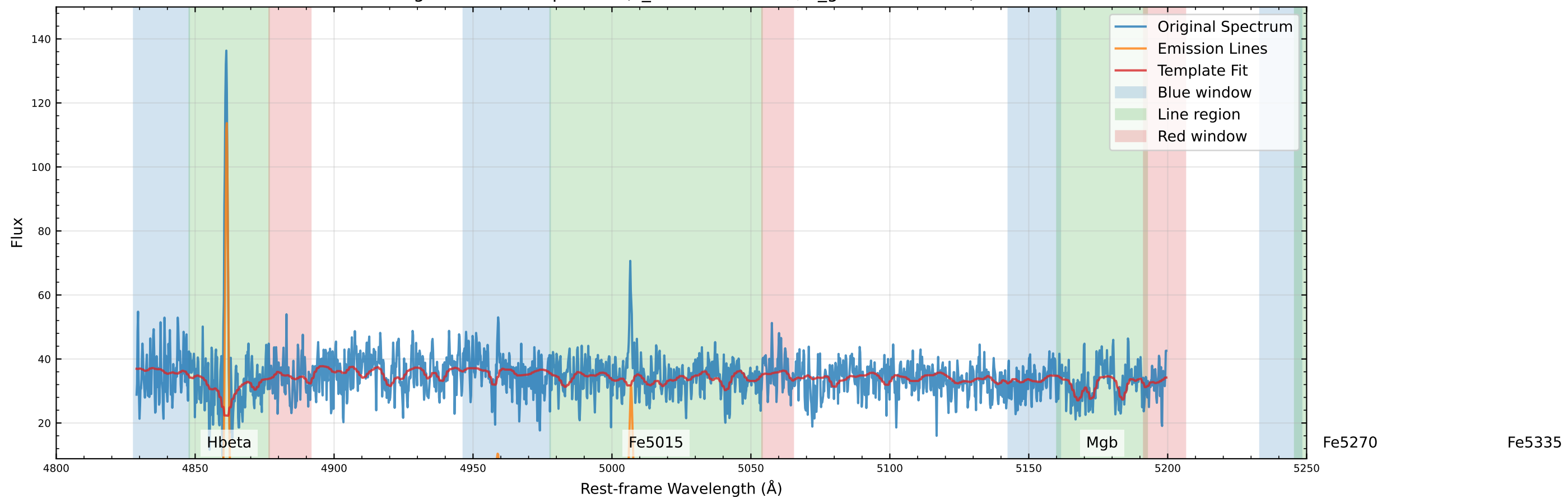
Original Data Comparison (v_star=-23.8 km/s, v_gas=-13.4 km/s)
