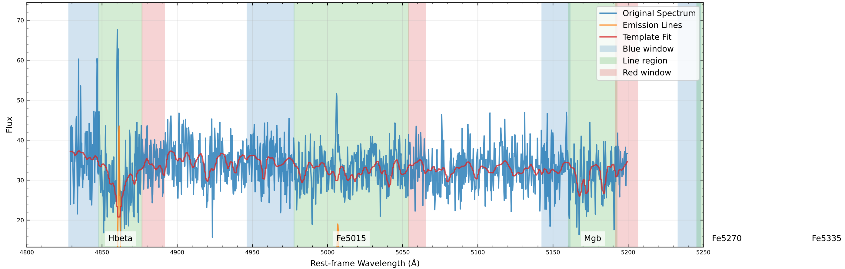
Original Data Comparison (v_star=-57.3 km/s, v_gas=-54.8 km/s)
