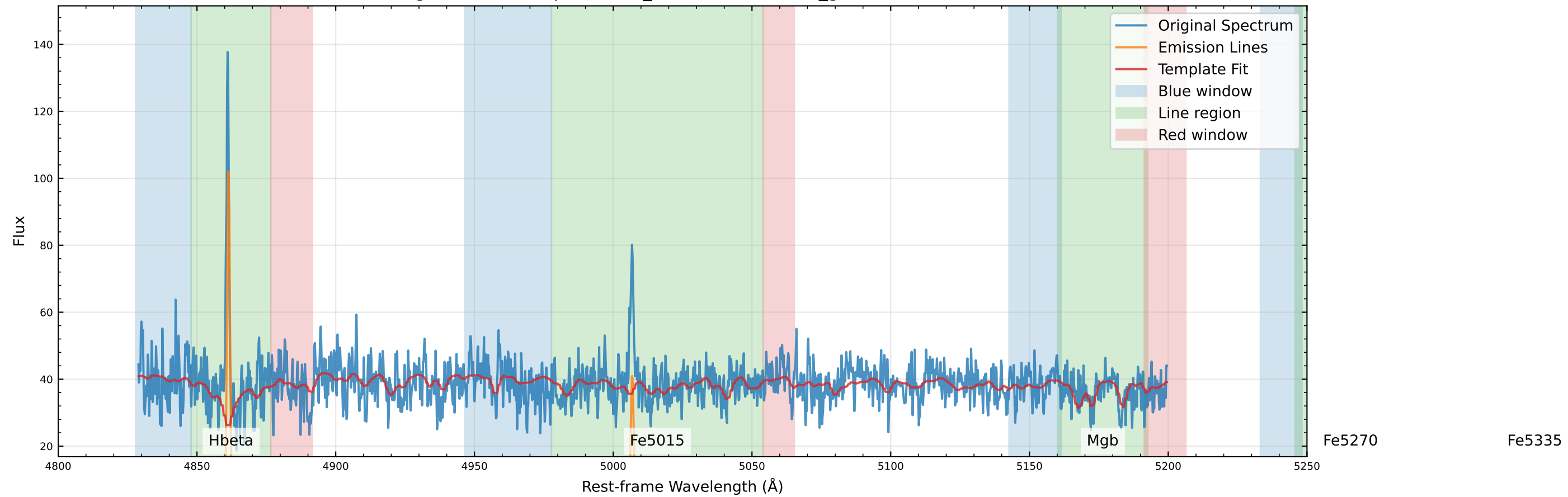
Original Data Comparison (v_star=-25.0 km/s, v_gas=-16.9 km/s)
