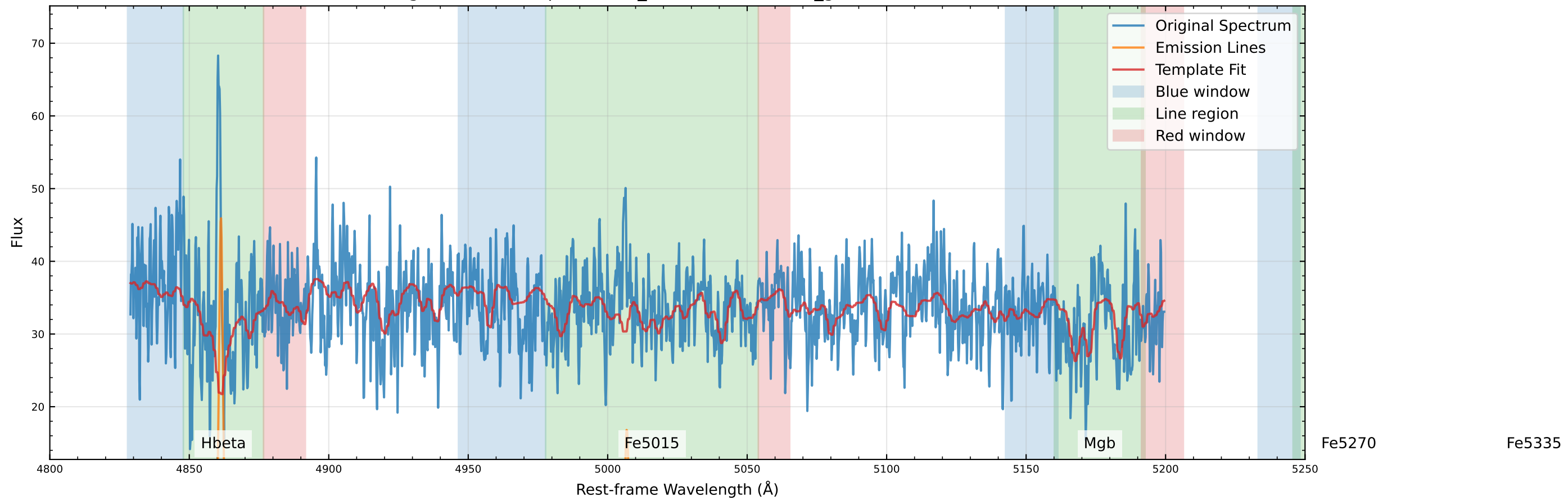
Original Data Comparison (v_star=-52.2 km/s, v_gas=-50.0 km/s)
