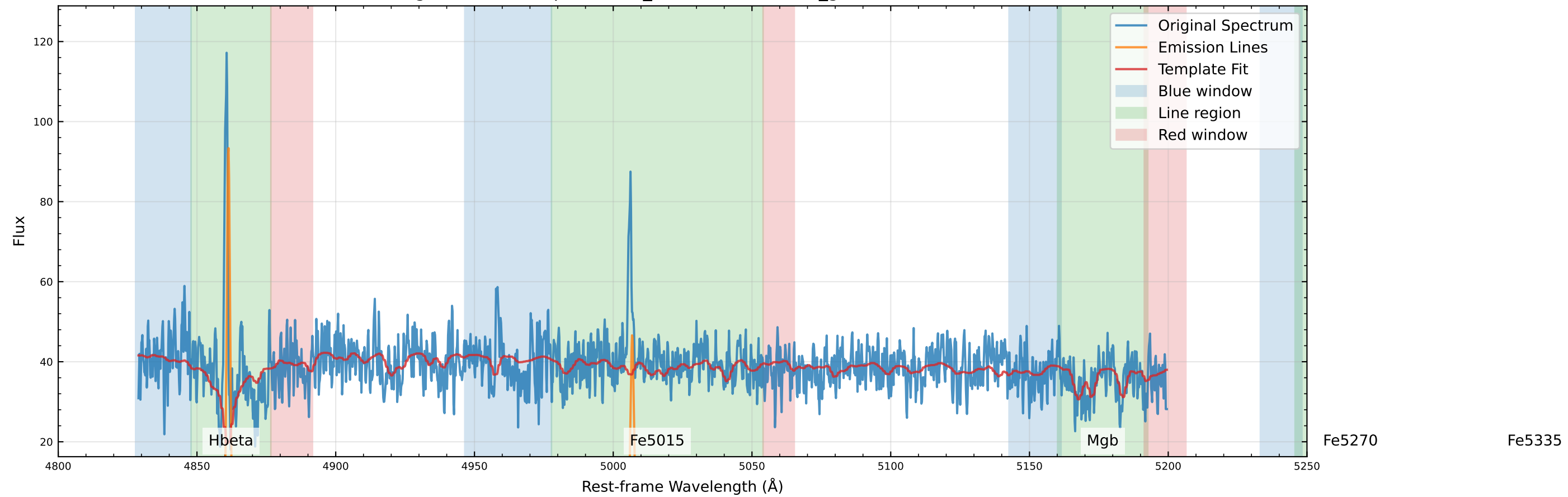
Original Data Comparison (v_star=-47.6 km/s, v_gas=-51.2 km/s)
