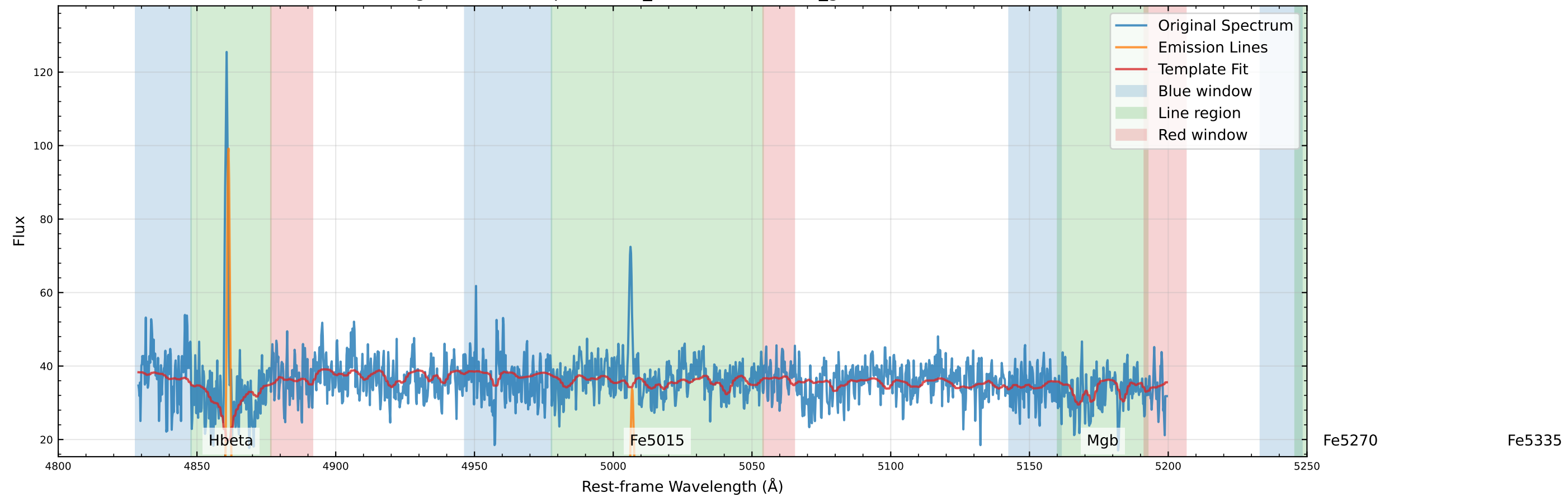
Original Data Comparison (v_star=-72.9 km/s, v_gas=-41.2 km/s)
