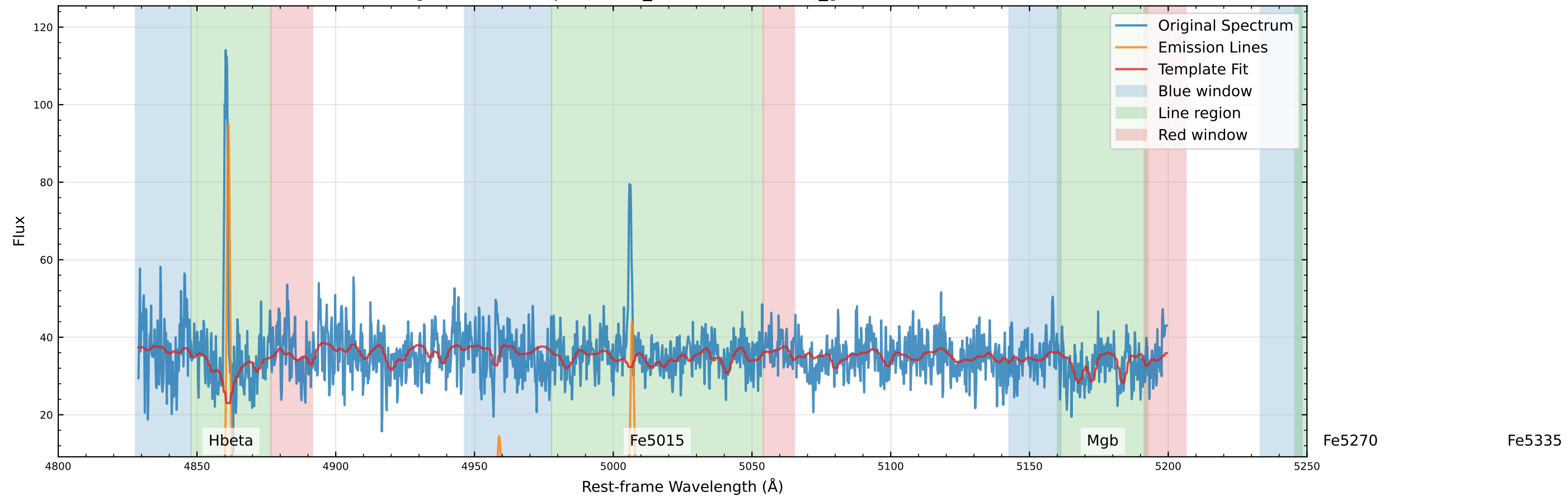
Original Data Comparison (v_star=-62.0 km/s, v_gas=-51.5 km/s)
