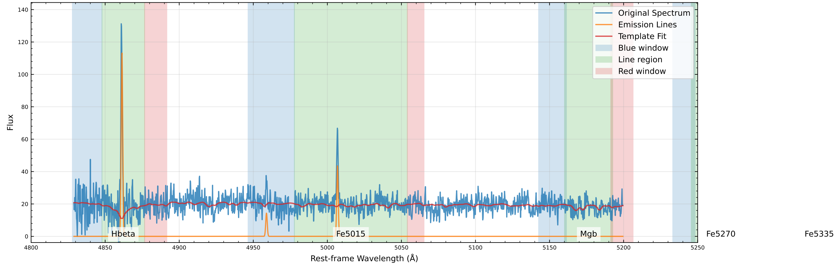
Original Data Comparison (v_star=-26.4 km/s, v_gas=-14.0 km/s)
