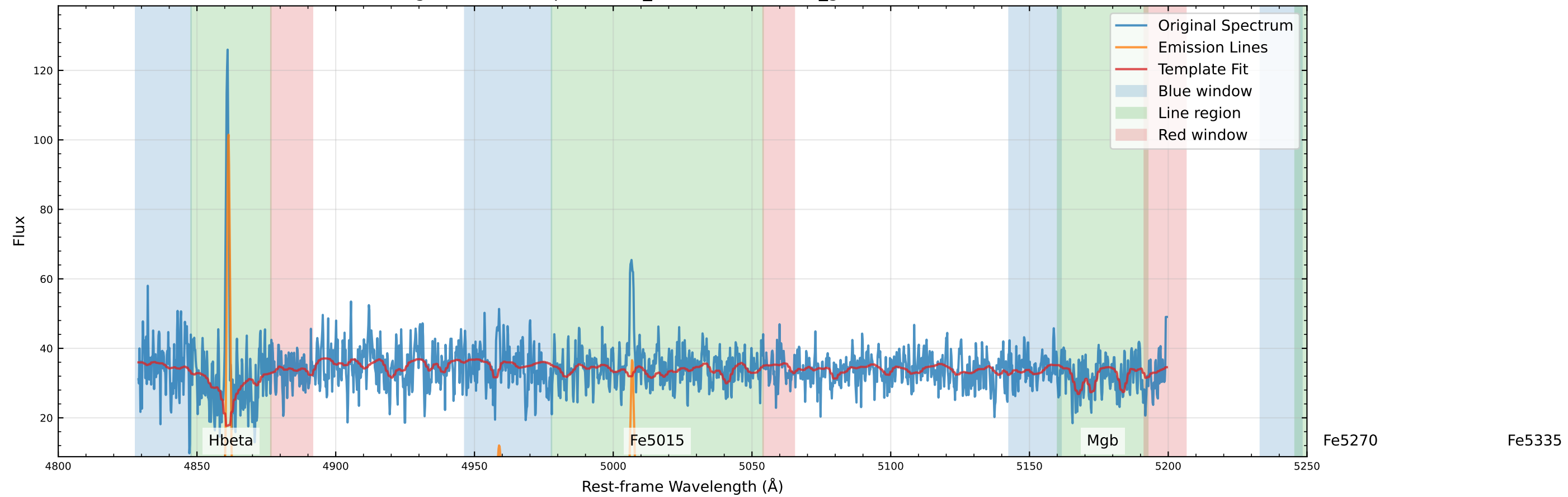
Original Data Comparison (v_star=-45.3 km/s, v_gas=-24.7 km/s)
