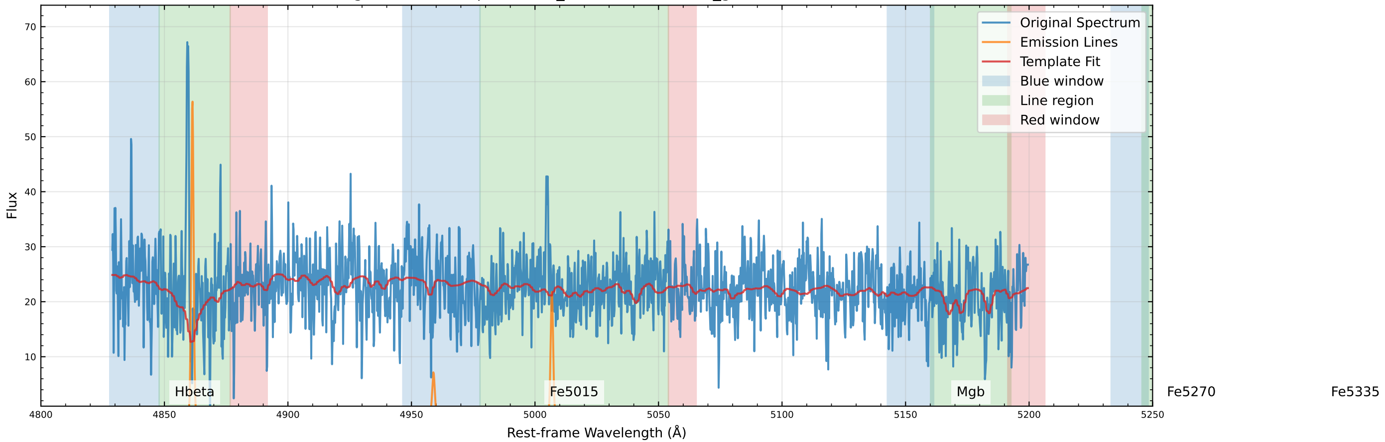
Original Data Comparison (v_star=-90.2 km/s, v_gas=-119.8 km/s)
