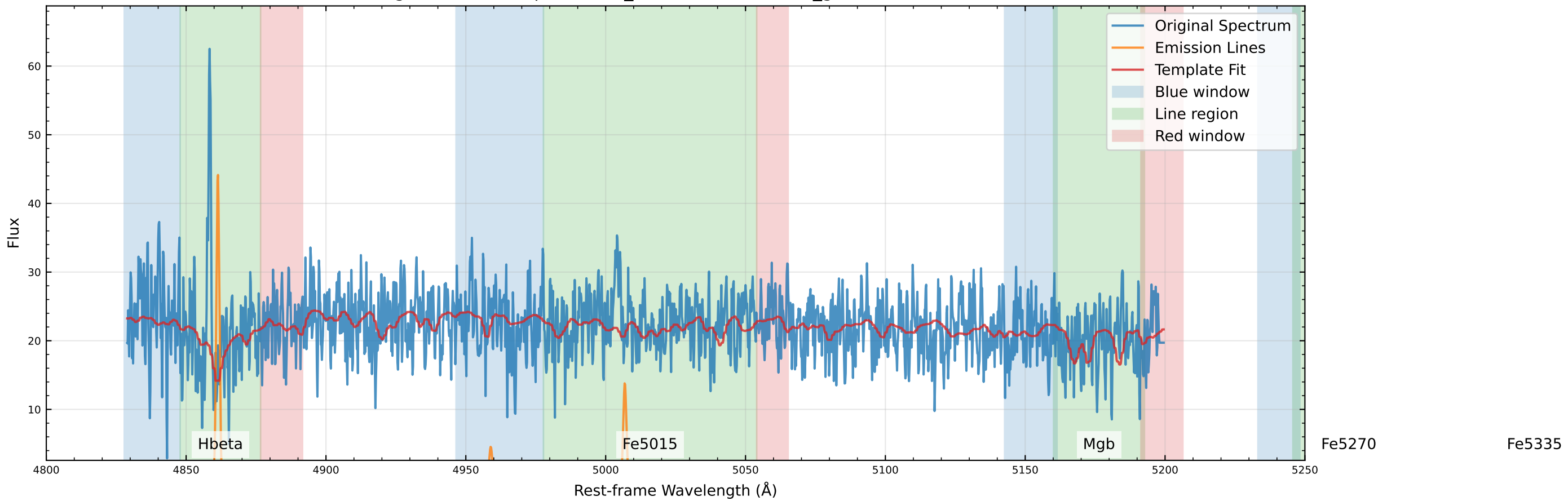
Original Data Comparison (v_star=-186.7 km/s, v_gas=-183.0 km/s)
