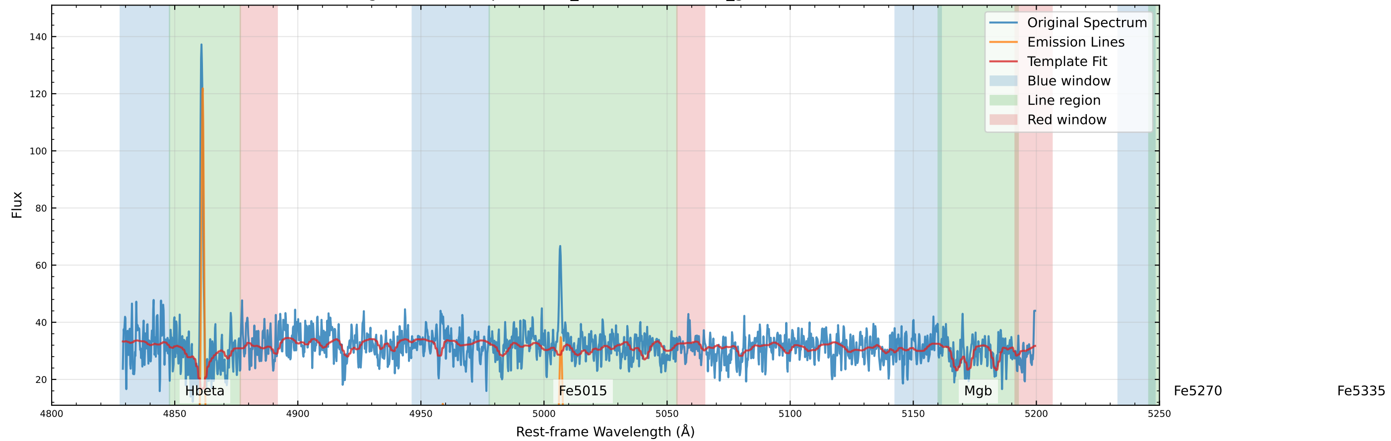
Original Data Comparison (v_star=-49.9 km/s, v_gas=-23.5 km/s)
