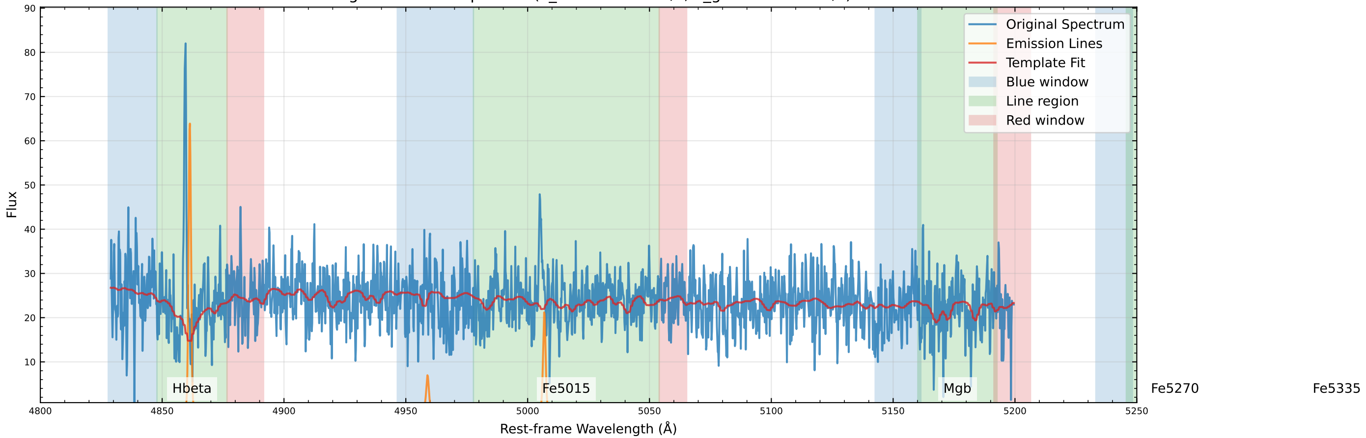
Original Data Comparison (v_star=-82.6 km/s, v_gas=-114.4 km/s)
