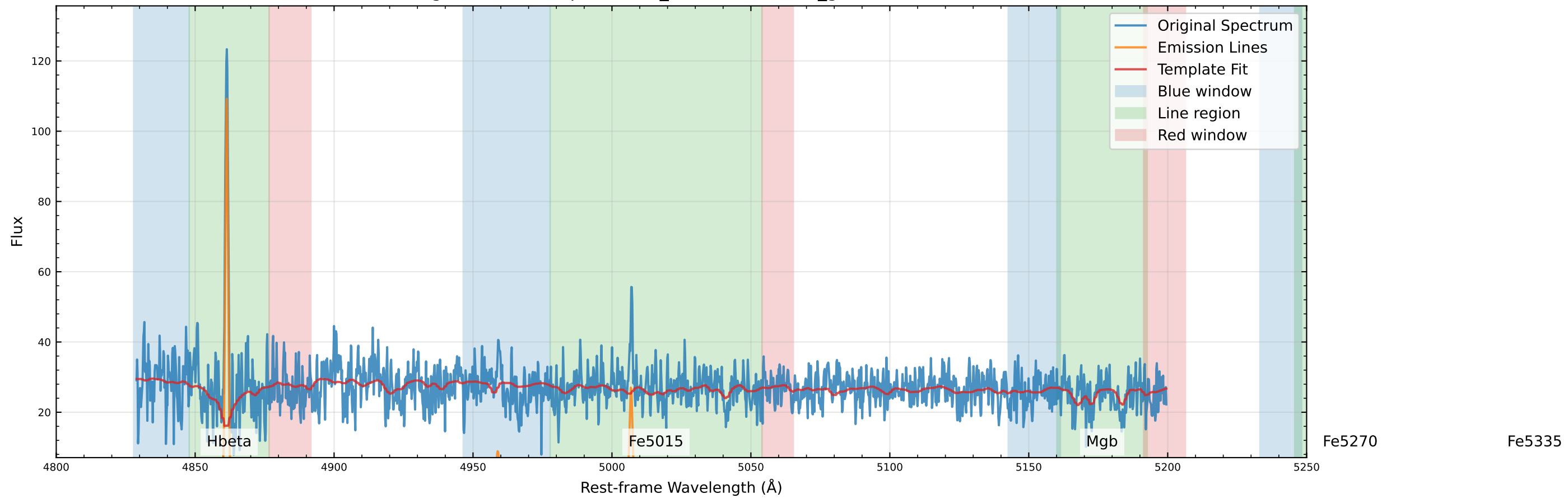
Original Data Comparison (v_star=8.3 km/s, v_gas=0.3 km/s)
