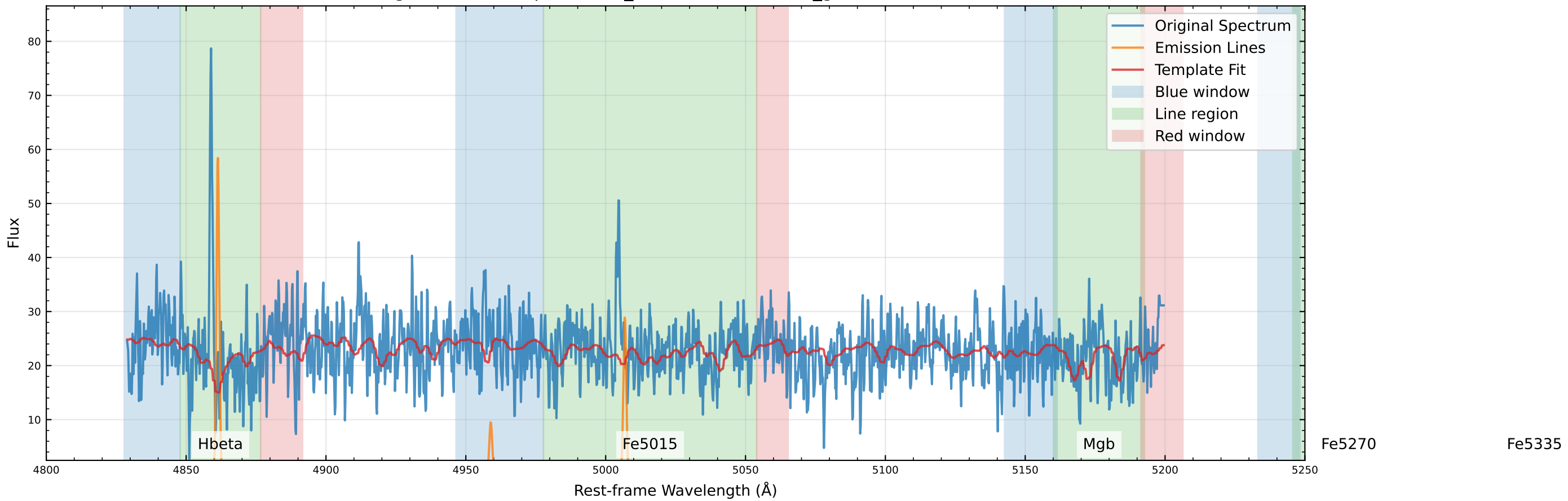
Original Data Comparison (v_star=-140.5 km/s, v_gas=-147.9 km/s)
