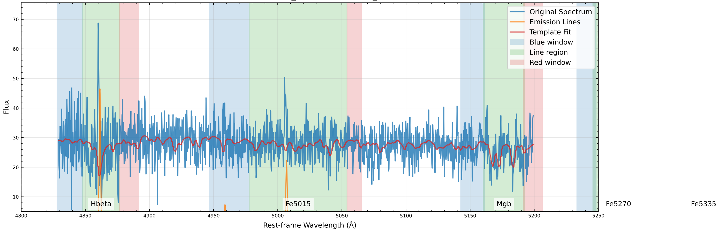
Original Data Comparison (v_star=-63.4 km/s, v_gas=-75.5 km/s)
