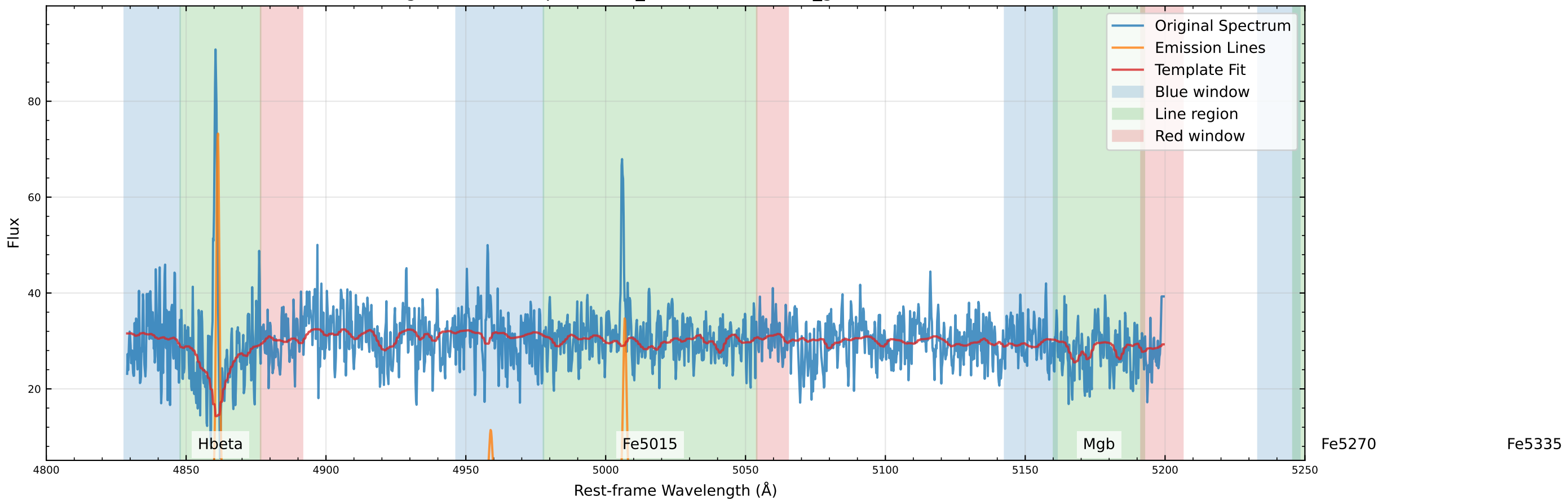
Original Data Comparison (v_star=-89.1 km/s, v_gas=-52.8 km/s)
