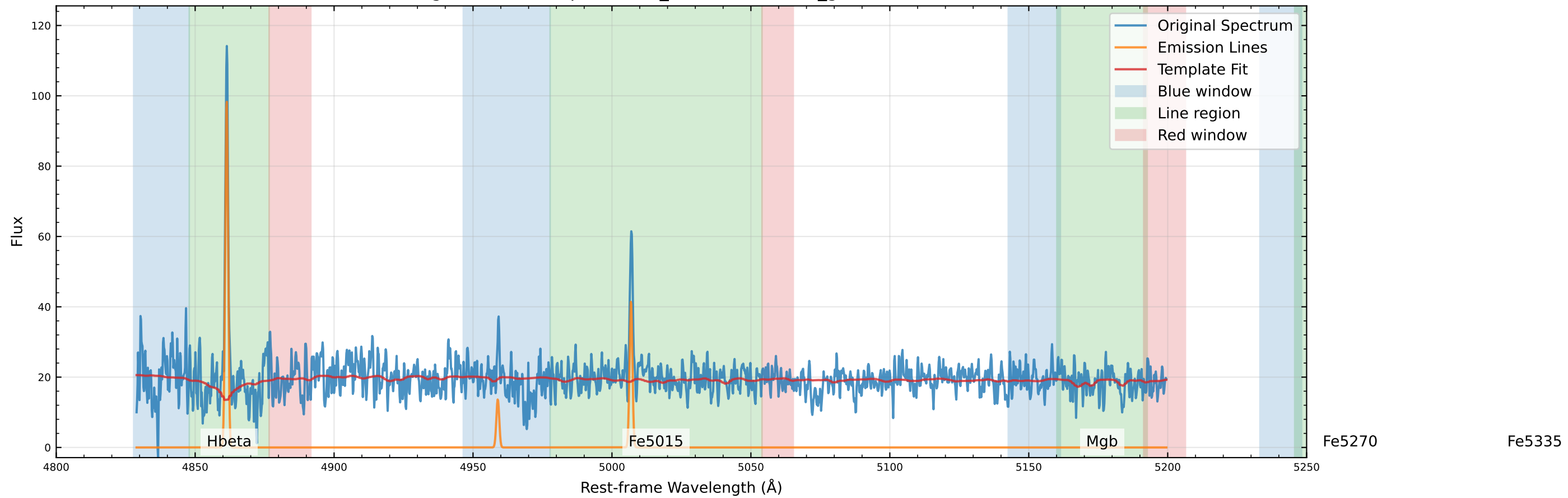
Original Data Comparison (v_star=4.1 km/s, v_gas=2.1 km/s)
